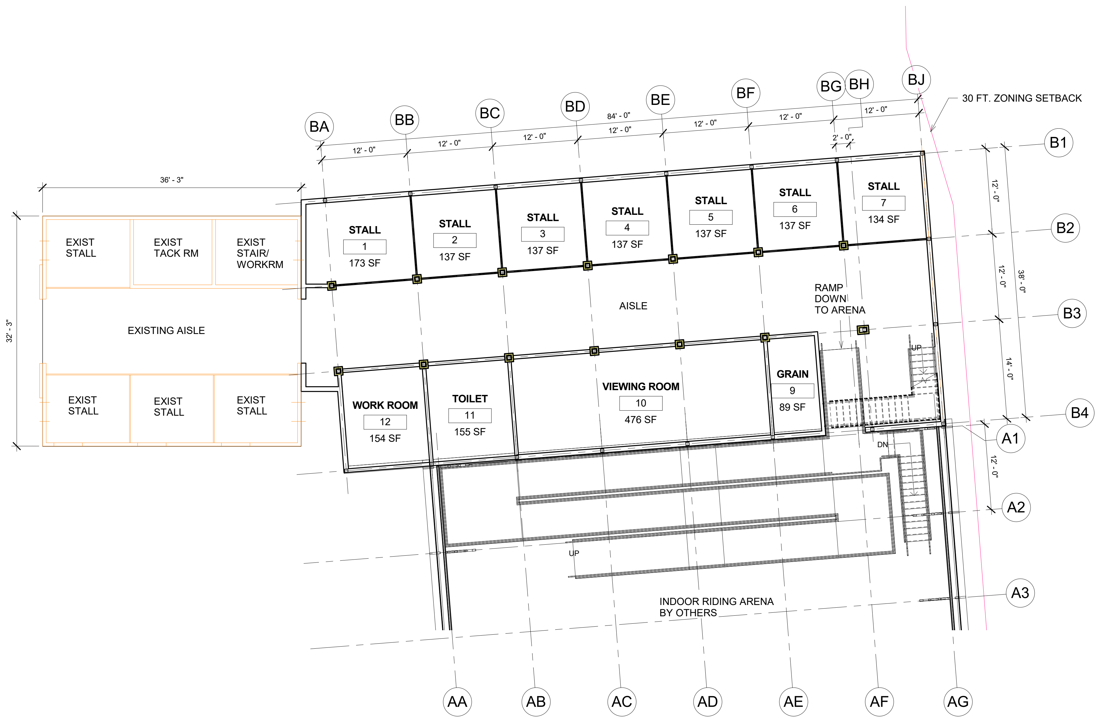
1 BARN LEVEL 1 - ENLARGED 1/8" = 1'-0"
